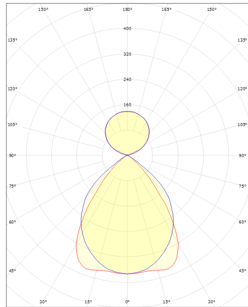
cd/klm \eta = 100\% — C0/C180 — C90/C270
