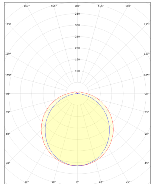
cd/klm — C0/C180 — C90/C270 η = 100 %
