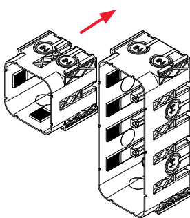
Sammenkobling
